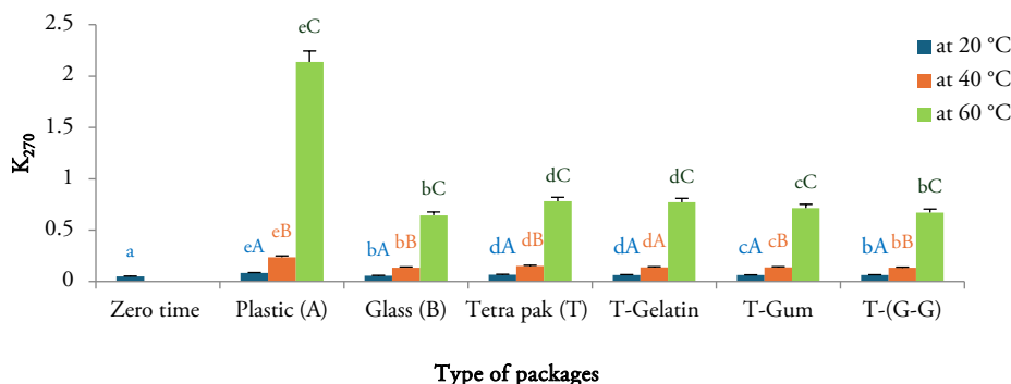
Figure 9. Influence of Storage Temperature on K 270 of Olive Oil in Different Packages after Eight Weeks a, b, c, d, e, f, and g are used to compare means of results for types of packaging after storage time. A, B, C are used to compare means of results at each temperature after storage time. Mean values with different letters are significantly different ( p < 0.05 )
